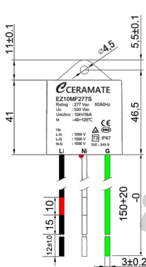
塑胶壳装灌胶防水型(分离线缆) Plastic casing and potting, waterproof(Separated wires) EZ10MF277S-S
