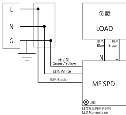
串联接法 Series Connection
