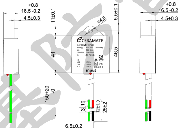
塑胶壳装灌胶防水型(护套软电缆) Plastic casing and potting, waterproof(Sheathed Flexible Cable) EZ10MF277S-C
