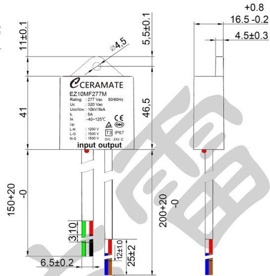
塑胶壳装灌胶防水型(护套软电缆) Plastic casing and potting, waterproof(Sheathed Flexible Cable) EZ10MF277M-C
