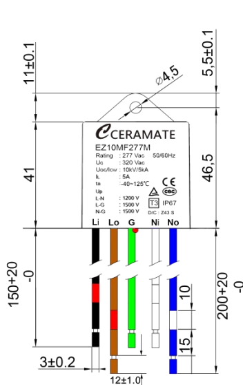
塑胶壳装灌胶防水型(分离线缆) Plastic casing and potting, waterproof(Separated wires) EZ10MF277M-S
